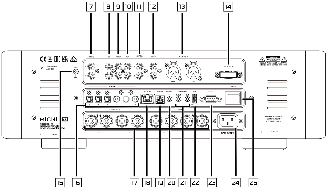
Figure 1_2: Controls and Connections Commandes et Branchements Bedienelemente und -Anschlüsse Controlles y Conexiones
