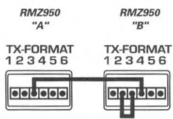
Use this jumper arrangement in a system with 2 RMZ950 controllers to disable the flood IR emitters on the first controller and enable the emitter on the second.
