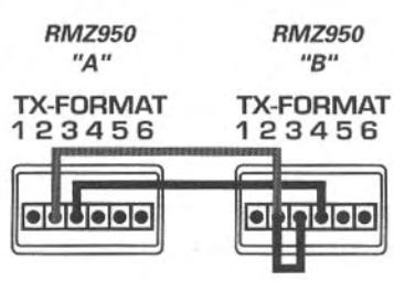
Use this jumper arrangement in a system with 2 RMZ950 controllers to enable the flood IR emitters on both RMZ950 controllers.
