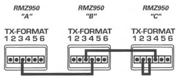
Use this jumper arrangement in a system with 3 RMZ950 controllers to disable the flood IR emitters on the first two controllers and enable the emitter on the third.
