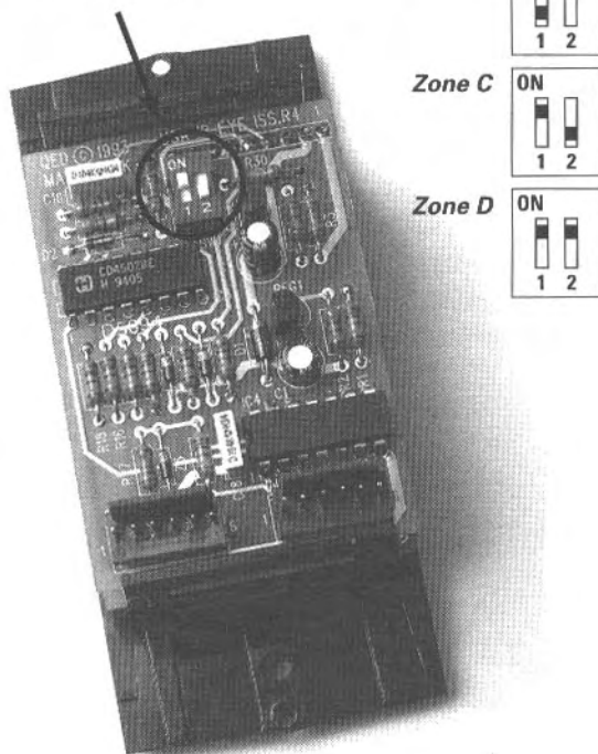
Zone switches
