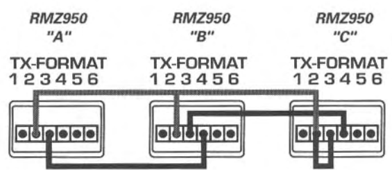
Use this jumper arrangement in a system with 3 RMZ950 controllers to activate the flood IR emitters on all three RMZ950 controllers.
